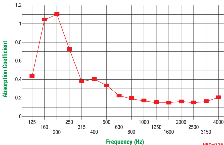
Decoustics Sound Absorption Data ME/LFTX2 (FR 701). Type F5 Mounting
